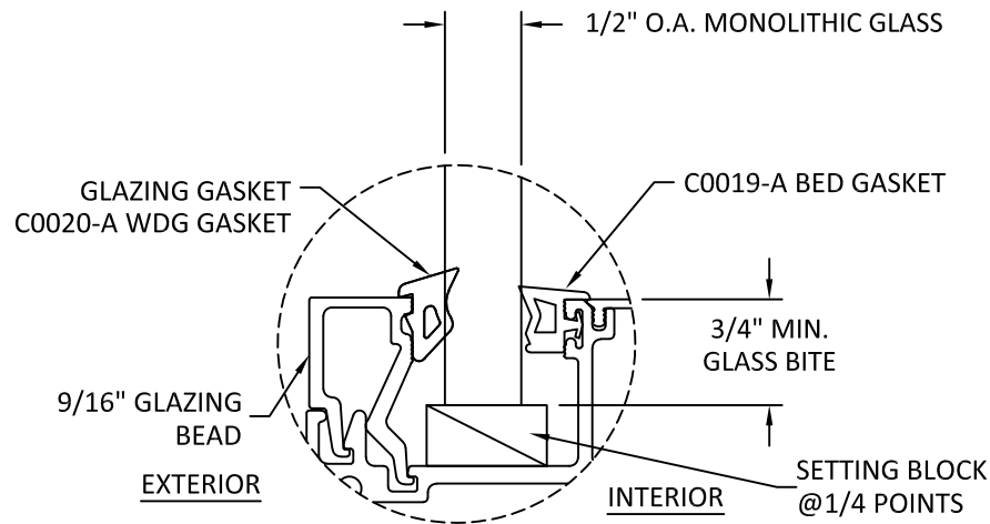
GLAZING DETAIL 1
