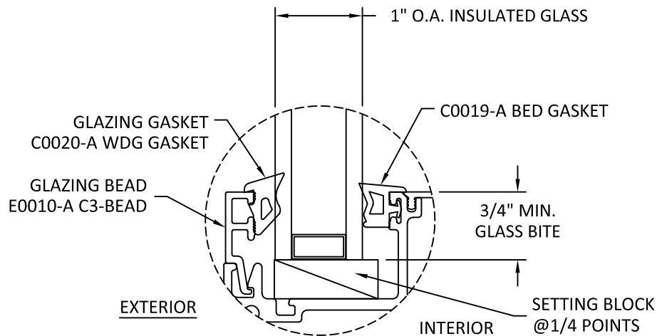
GLAZING DETAIL 2
